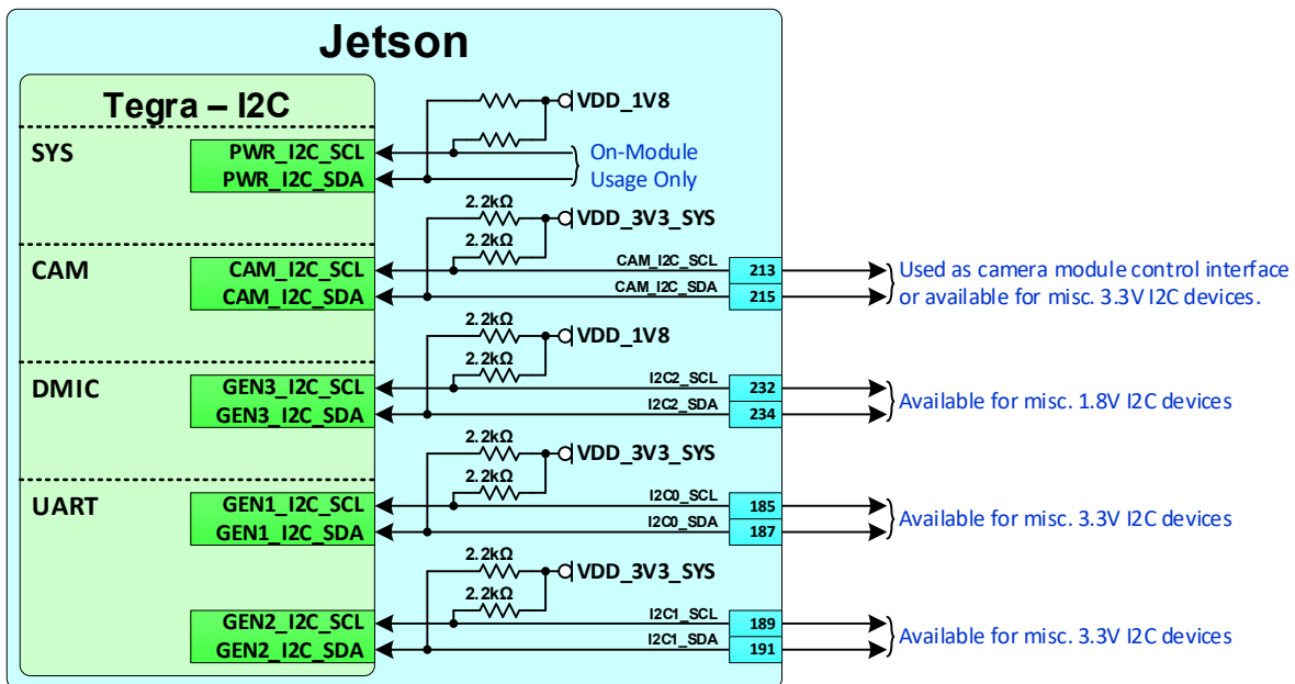
Figure 11-1. I2C Connections
